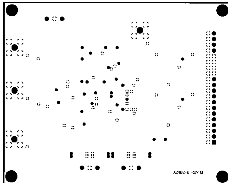
FIGURE 3. Power Plane.
